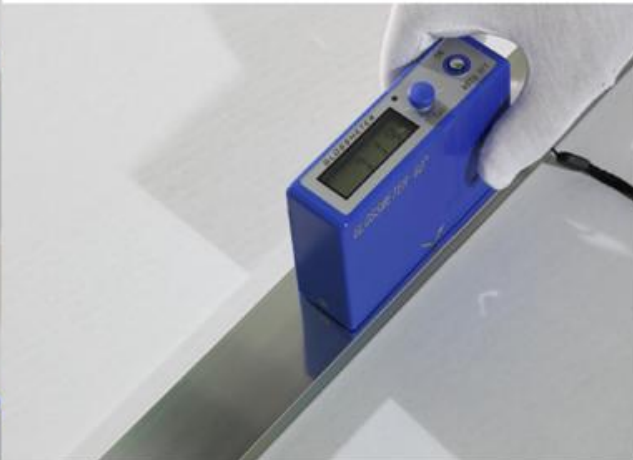
aluminium profile chrome gloss/brightness testing
