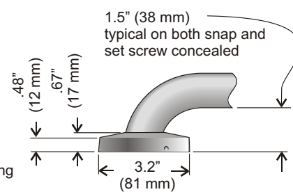
Snap flange dimensions
